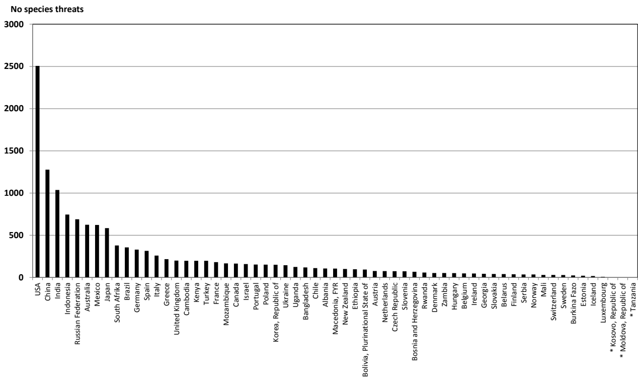
Figure 19. Species threats, domestic, 2012 Data source: Lenzen et al. (2012). No data for Kosovo, Moldova and Tanzania.
