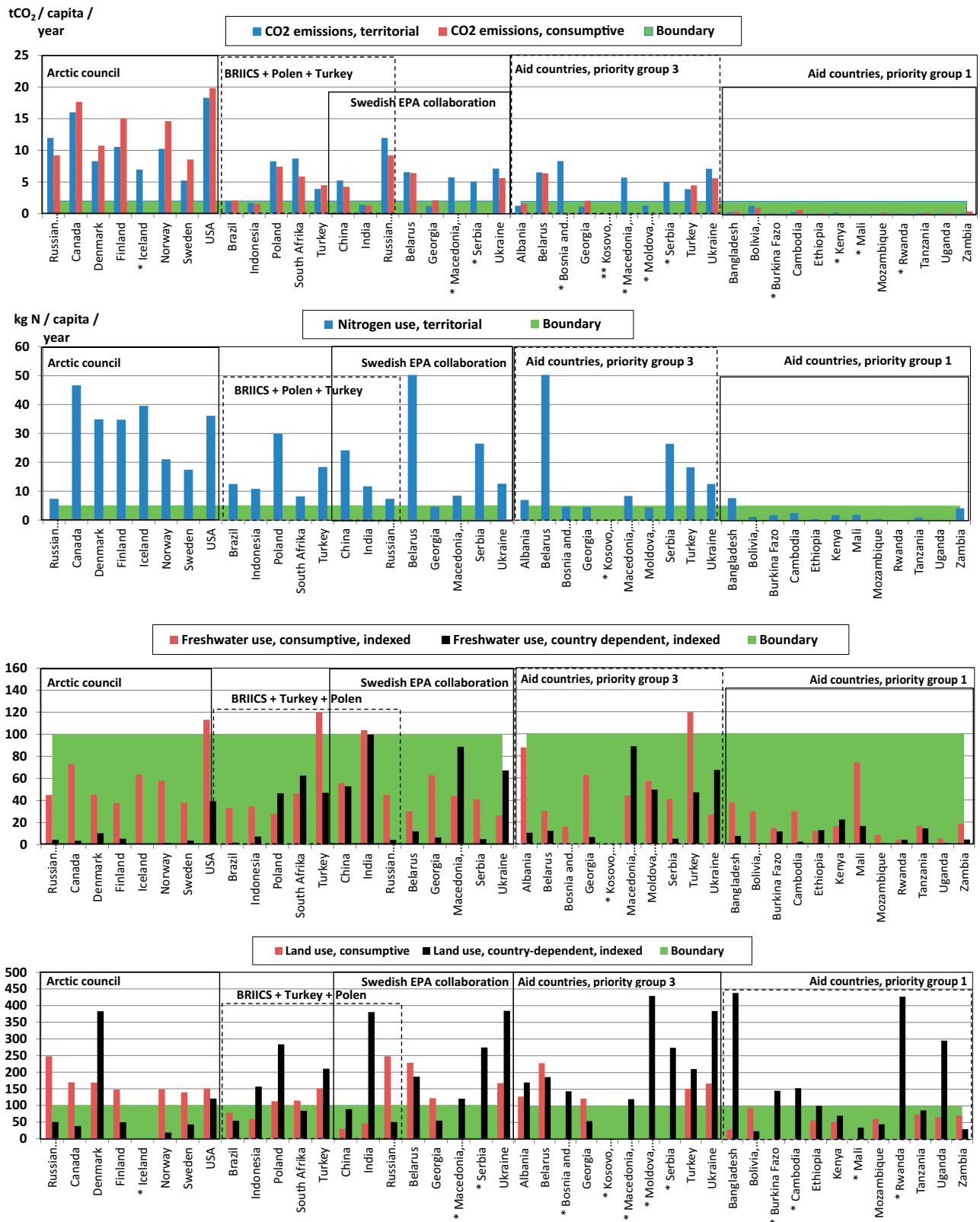
Figure 24. Comparing the performance of groups of countries on quantified national boundaries For Freshwater and Land use, results are shown in relation to country-dependent boundaries (i.e., related to national resource base). Note that for nitrogen use, only the territorial performance is used. *No data for Kosovo, and data are lacking for consumptive performance on Climate Change and Land Use for Moldova, Serbia, Iceland and several of the countries in aid category 1 (see above).
