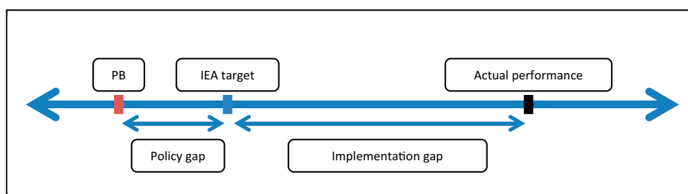
Figure 26. Illustration of policy gap vs. implementation gap
