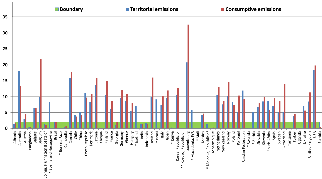
Figure 9. Climate change per capita boundary performance in 2008
