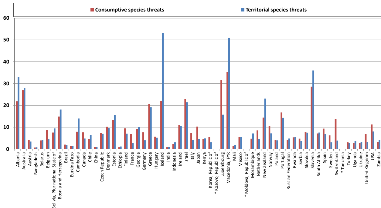
Figure 18. Biodiversity loss: performance on species threats per million capita, territorial and consumptive, 2012 Data source: Lenzen et al. (2012) based on IUCN species listed as “threatened”, shown as per million capita. *No data for Kosovo, Moldova and Tanzania.
