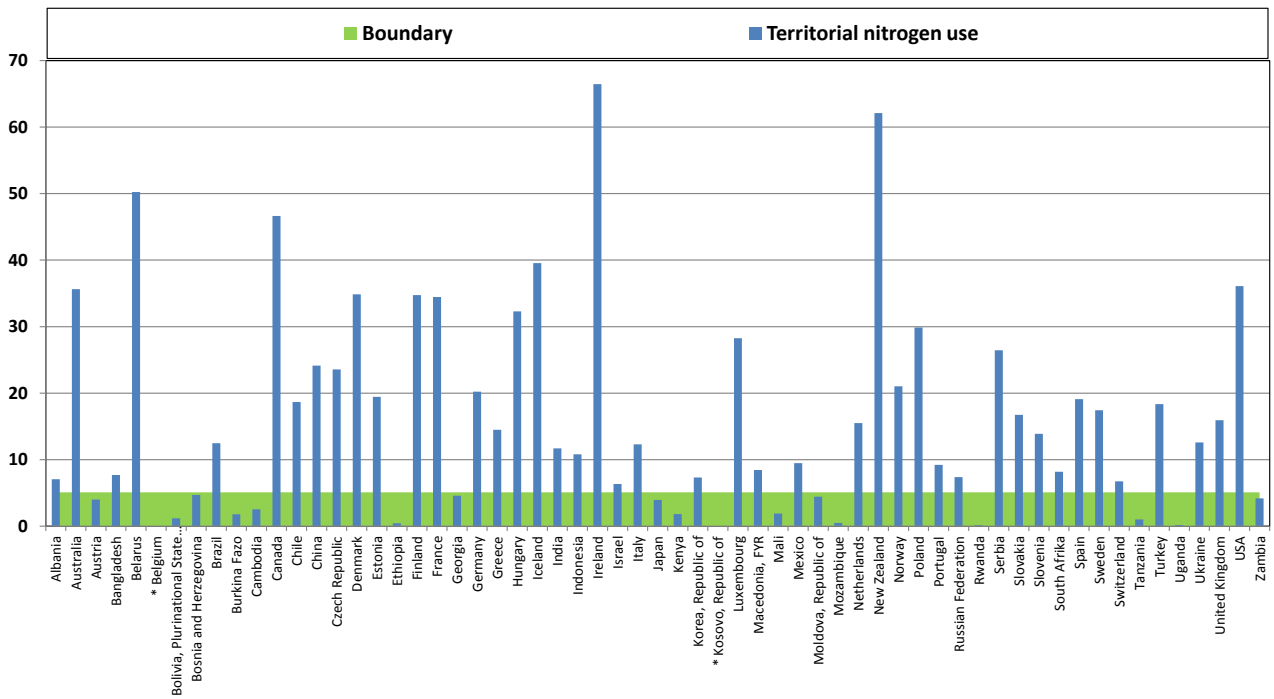
Figure 11. Nitrogen: territorial performance on per capita boundary, average of 2005–2009 Data source: FAO (2012), an average of 2005–2009 is used due to the variability of the data. *No data for Kosovo and Belgium.
