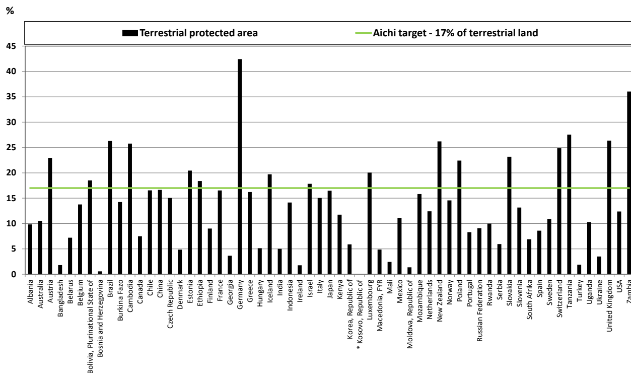
Figure 21. Terrestrial protected areas in 2010 and Aichi biodiversity target 11 Data source: World database on protected areas. *No data for Kosovo.
